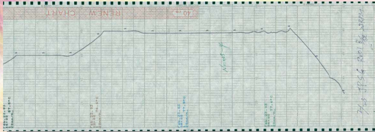
製程持溫段溫度控制在 ± 0.2 度反應性穩定良好 Constant temperature range is controlled within 0.2°C, ensuring stable chemical reactions.
