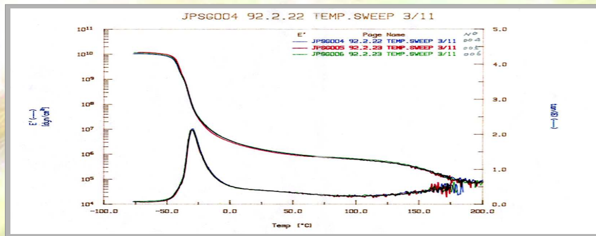
水性膠帶糊產品取樣作DMA(Dynamic Mechanical Analyzer 機動態分析)分析圖曲線重疊一致，批間品質相當穩定 Dynamic Mechanical Analysis (DMA) is conducted on water-based Acrylic PSA. The analysis curve is consistent, showing steady inter-batch quality.
